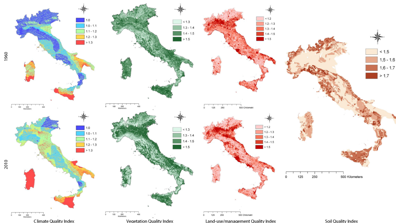
Fig. 2. Spatial distribution of the average ESA scores of the four partial indicators (CQI, VQI, MQI, SQI) in Italy at the beginning and the end of the study period.
