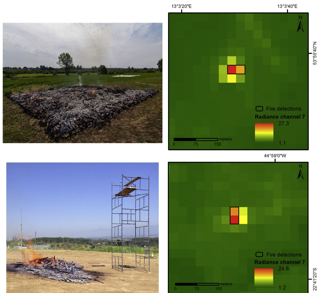
Fig. 7. Experimental fires used in support of Landsat-8 fire algorithm verification. The two rows show photos of the sites (left panels), and the OLI channel 7 image subset of the area with fire pixels marked in black (right panels). Top panels describe the 11 \times 13 \text{ m}^2 plot near Demmin/Germany ( 53.9276^\circ \text{N} 13.0587^\circ \text{E} ) on 17 August 2013; bottom panels describe the 3 \times 10 \text{ m}^2 plot near Cachoeira Paulista/Brazil ( 22.6868^\circ \text{S} 44.9844^\circ \text{W} ) on 19 January 2015. (For interpretation of the references to color in this figure legend, the reader is referred to the web version of this article.)
