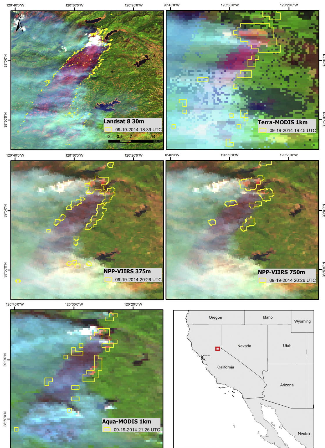
Fig. 5. Multi-sensor imaging of the King fire in California/U.S. on 19 September 2014. Active fire detections derived from Terra/MODIS 1 km, Landsat-8/OLI 30 m (path/row 43/33), S-NPP/VIIIRS 375 m and 750 m, and Aqua/MODIS 1 km are marked in yellow. Temporal separation between consecutive images was limited to approximately 1 h. (For interpretation of the references to color in this figure legend, the reader is referred to the web version of this article.)
