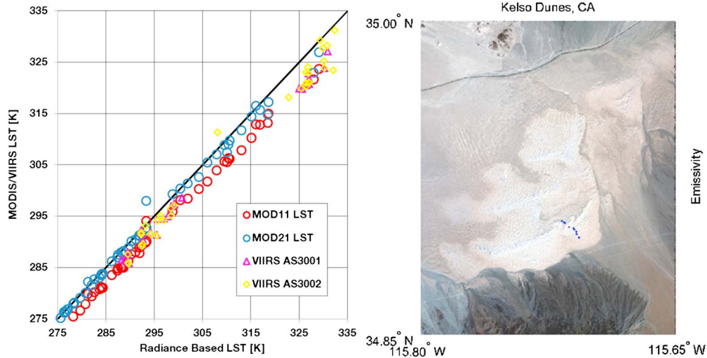
Figure 1. (left) Plot of MODIS/VIIIRS LST at the Kelso Dunes, California, pseudo-invariant site (image on right) versus radiance-based LST.
