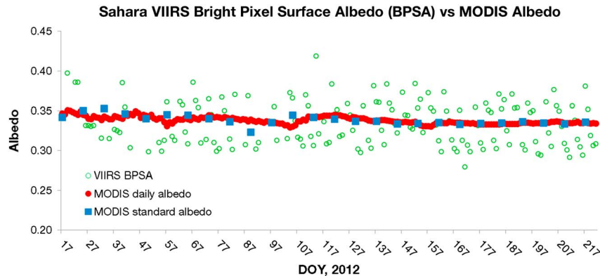
Figure 3. Comparison between VIIRS Bright Pixel Surface Albedo (BPSA) (green circles), MODIS Collection 5 eight-day standard product (blue squares), and MODIS Collection 6 daily albedo (analogous to the VIIRS Dark Pixel Surface Albedo (DPSA), red circles) over the Sahara site (a stable desert location: 26.450°N, 14.083°E) for 17 January to 4 August 2012. Daily BPSA varies between 0.29 and 0.40 in the Sahara. A recent look-up table (LUT) reduces this somewhat, but view-angle effects still dominate (LUT implemented 18 January 2013). A solution suggested to reduce variability is to simply implement a multiday average.
